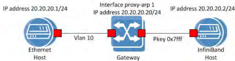
Figure 46: Basic Gateway Setup
