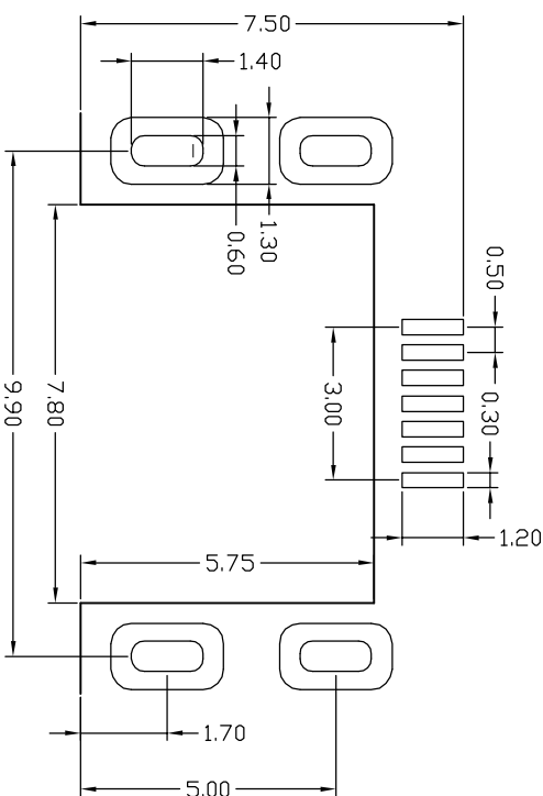
RECOMMENDED PCA LAYOUT
